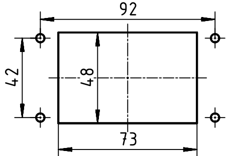
panel cut out (1:2)
